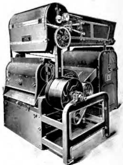
Improved Saw Gin with Feeder and Condenser.
