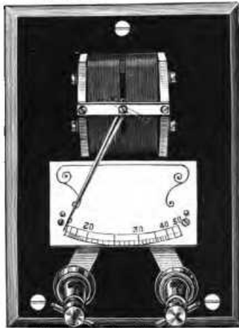
Astatic Ammeter, Cover removed.
