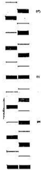
Fig. III.—About the Interference of Two Sound Waves.
